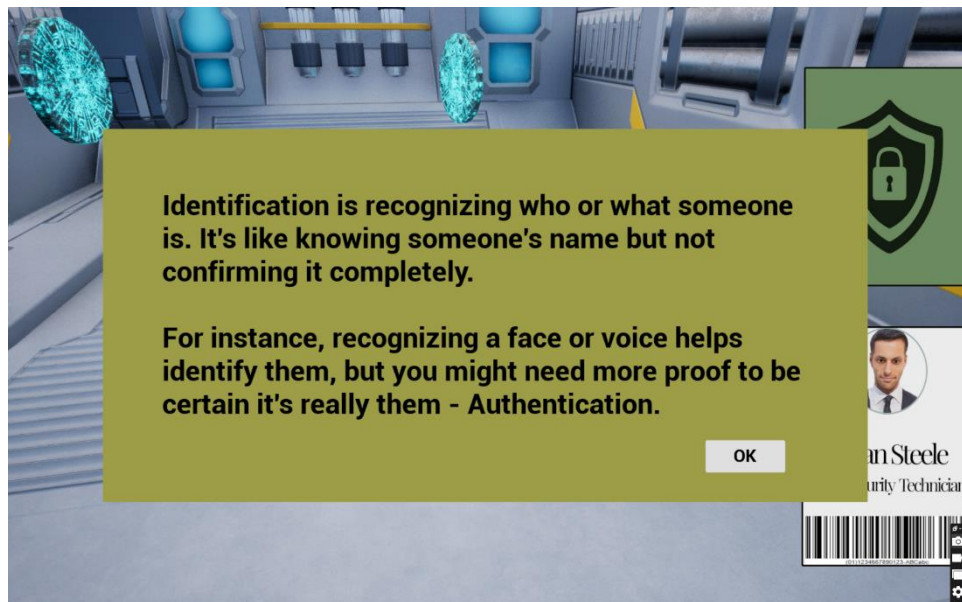
Figure 36 Identification Information
