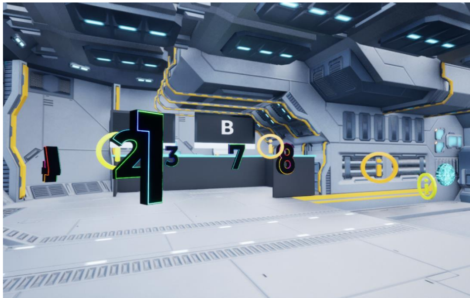
Figure 9 Level 1
