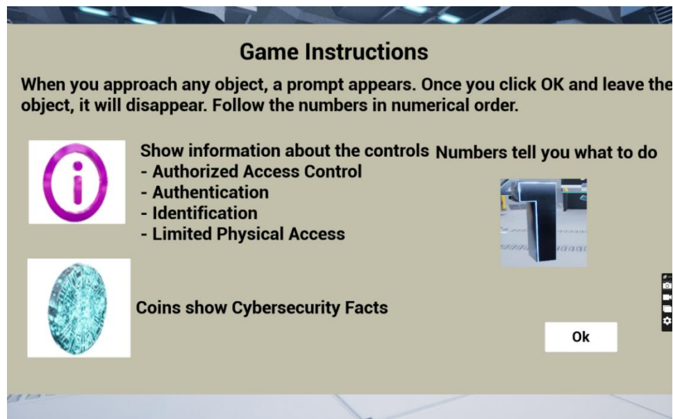
Figure 8 Game Instructions
