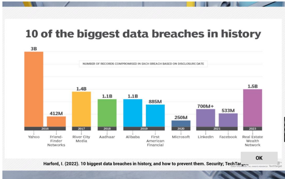
Figure 39 Breach Fact
