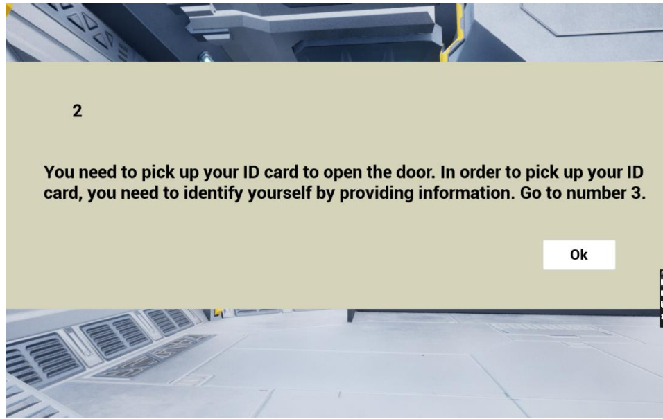
Figure 11 Second Prompt
