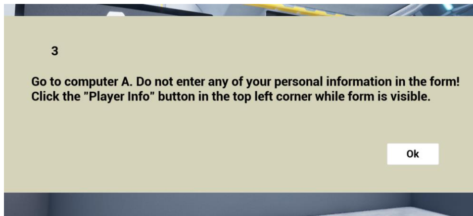
Figure 12 Third Prompt
