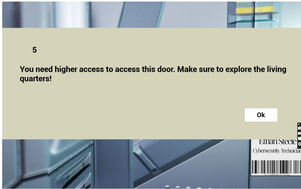
Figure 18 Fifth Prompt
