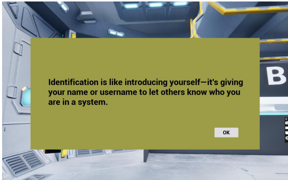
Figure 17 Identification Information
