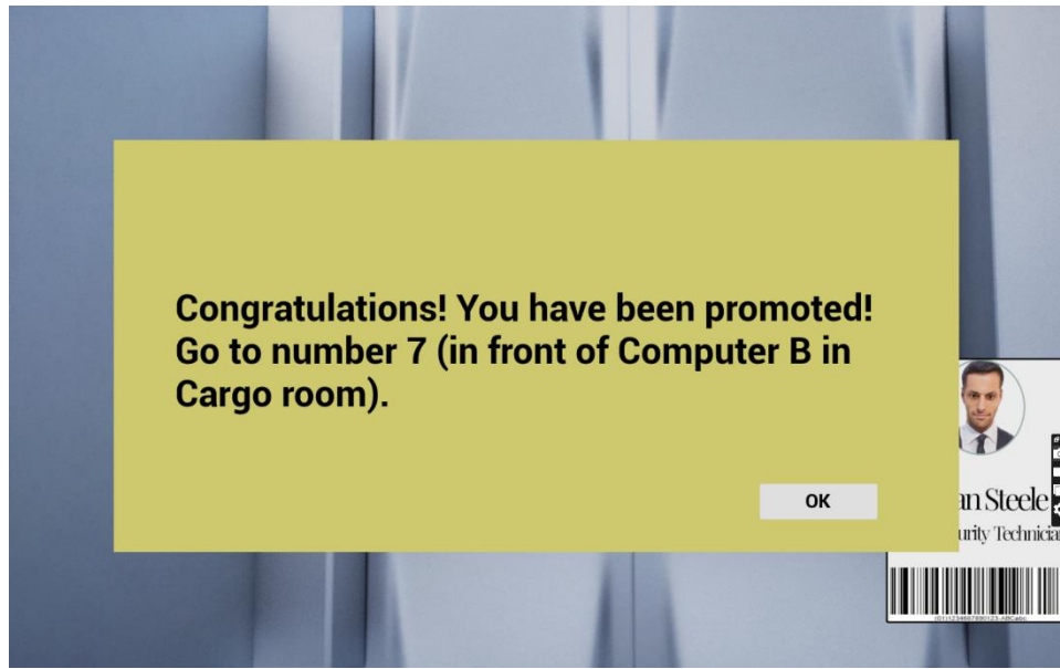
Figure 22 Promotion Prompt
