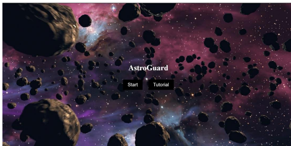
Figure 2 Main Screen
