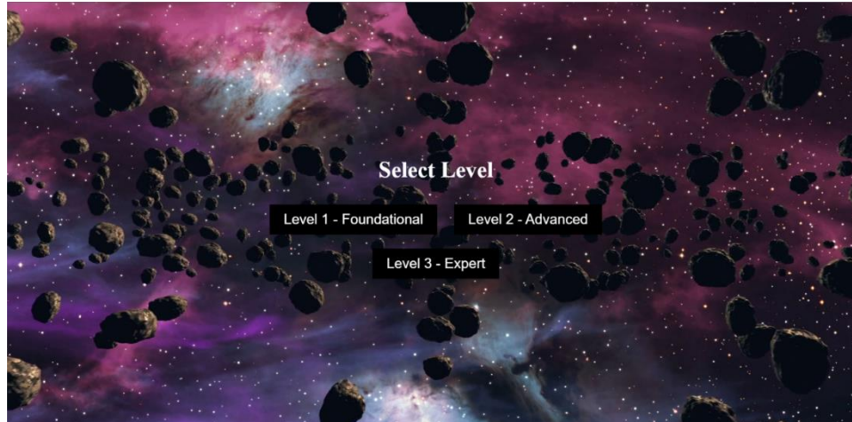
Figure 3 Level Screen
