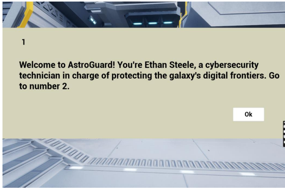
Figure 10 First Prompt
